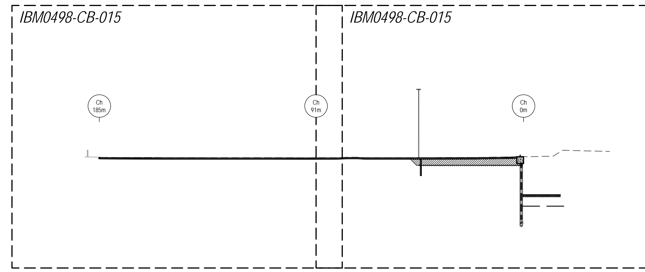
KEY: CROSSBERTH QUAY: SECTION F-F [1:1000]
