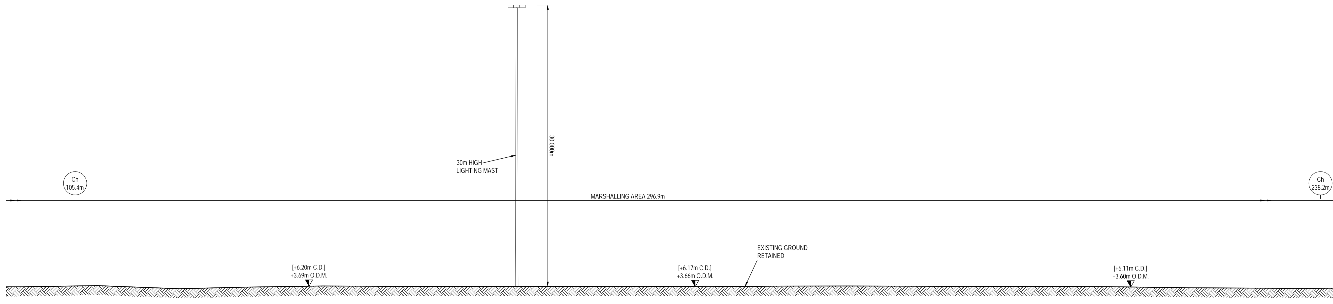
SECTION D-D: CHAINAGE 105.4m to 238.2m [1:200]
