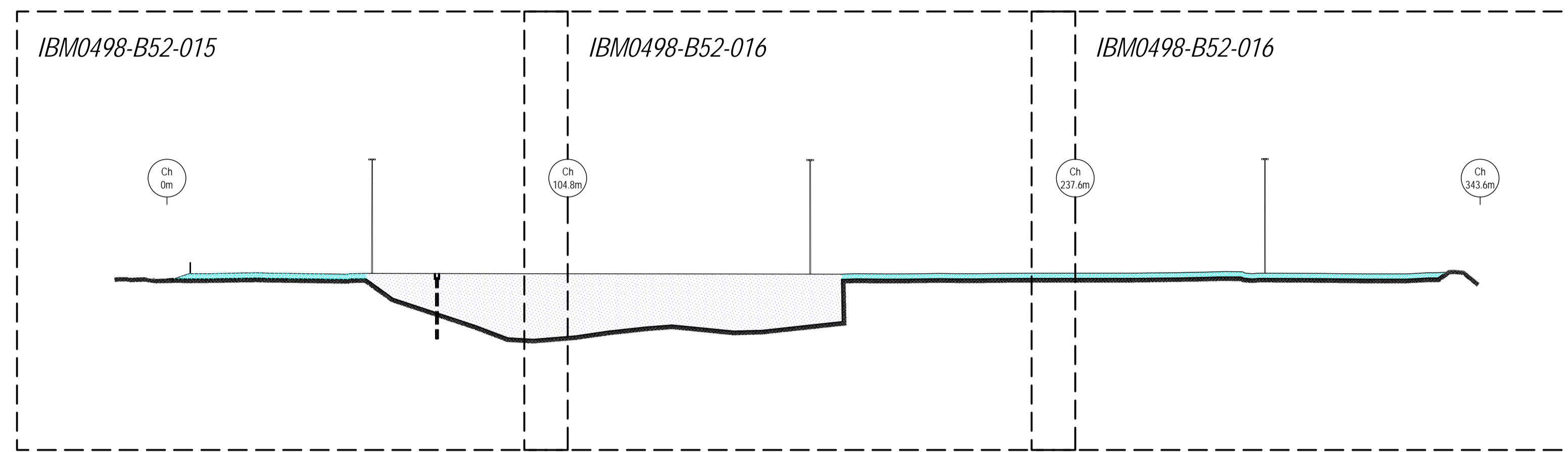
KEY: SECTION C-C NEW BERTH 52 WORKS [1:1,000]
